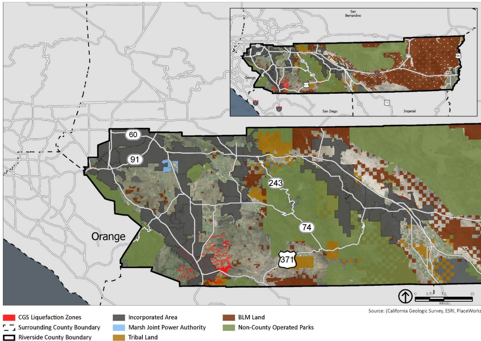
FIGURE 2: LIQUEFACTION ZONES
