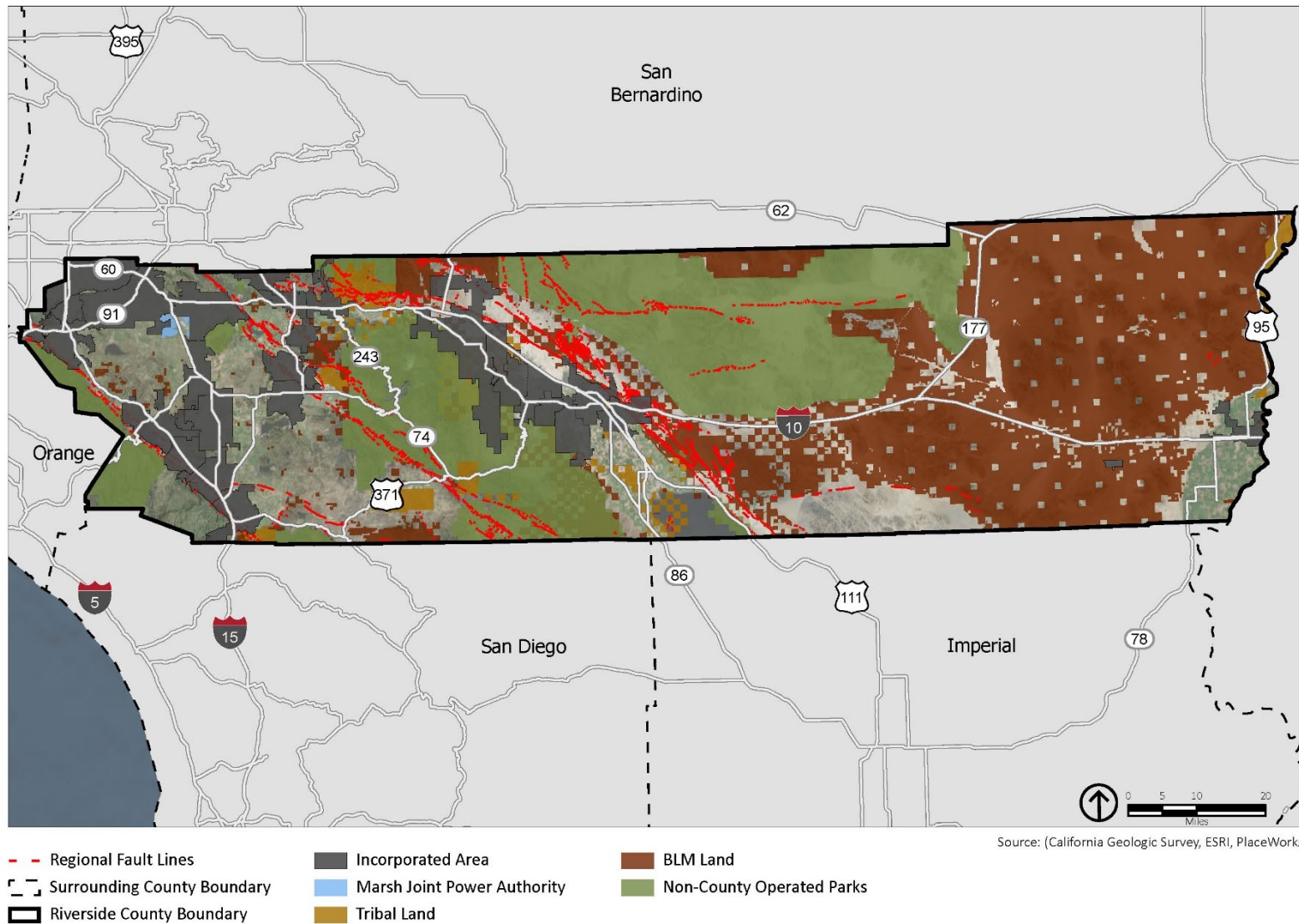
FIGURE 1: FAULT LINES
