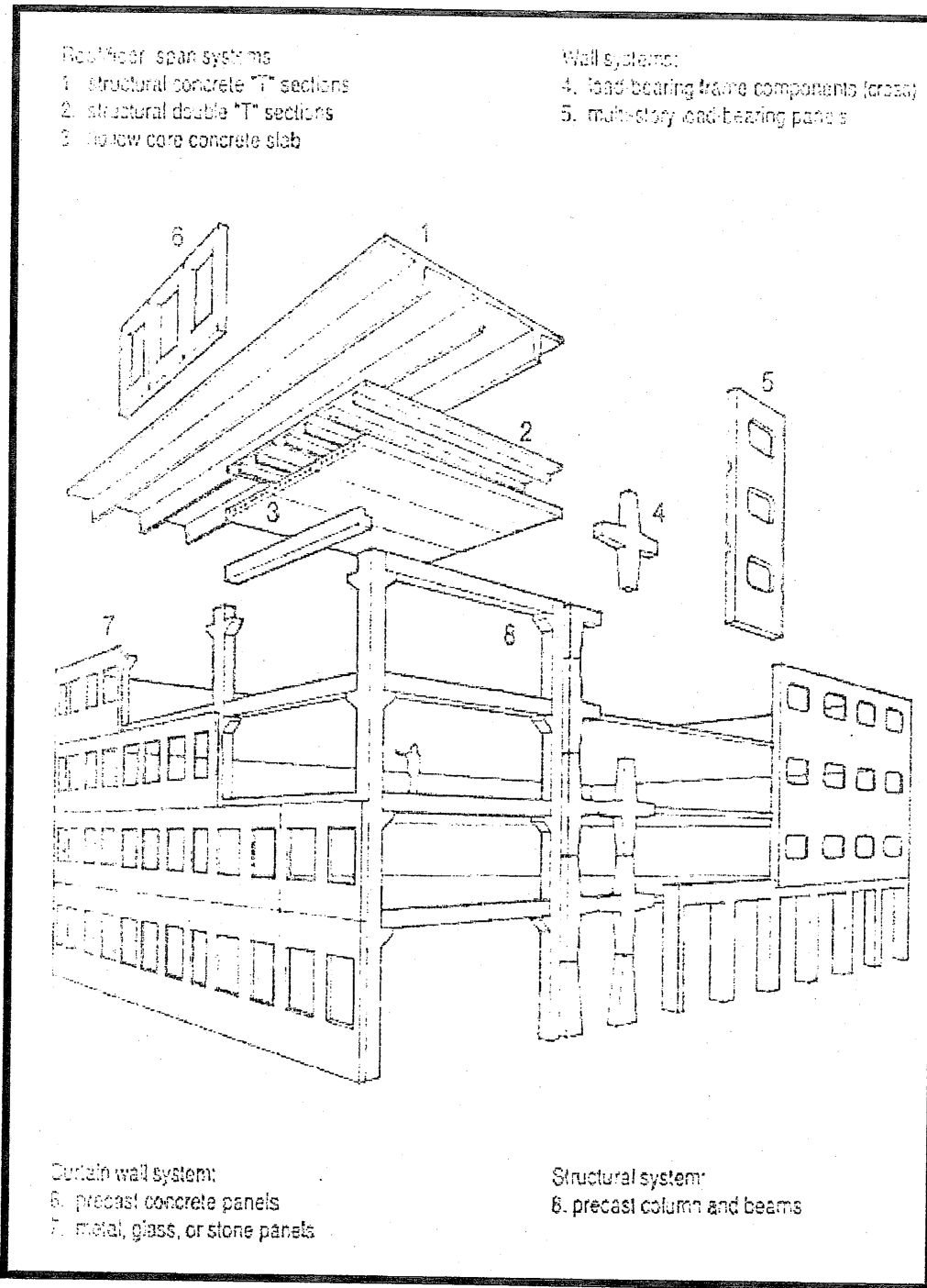
Figure 1-14: Precast concrete-frame construction. Prepared by the Applied Technology Council for the Federal Emergency Management Agency (1988), Rapid Visual Screening of Buildings for Potential Seismic Hazards: A Handbook: Earthquake Hazards Reduction Series 41, FEMA 154.
