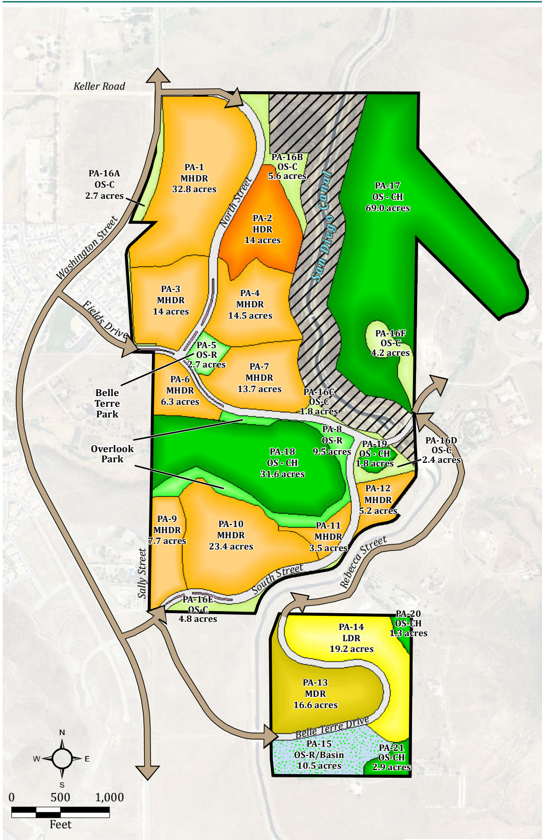
Figure A-1-1 Land Use Plan
